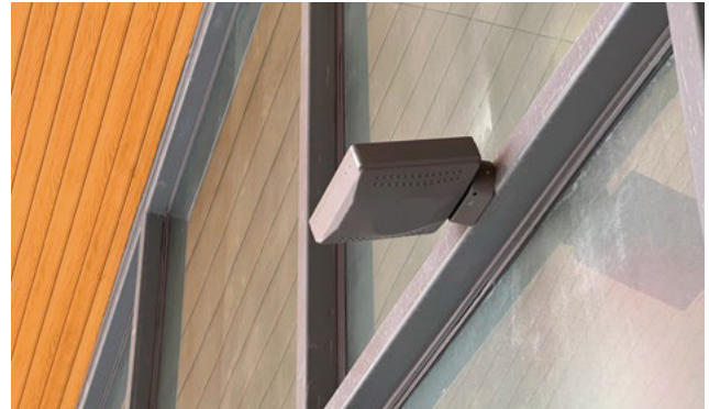
Equipped with junction box, it simplifies installation requirements and processes, providing convenience and safety assurance for projects. Whether it's narrow or wide spaces, the split installation bracket can easily cover all demands
